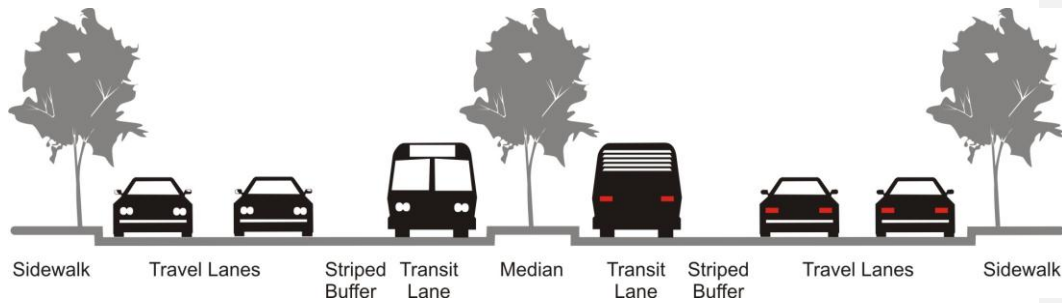
Figure 6 Recommended Corridor Segment Treatment: Two-Lane Side Busway
