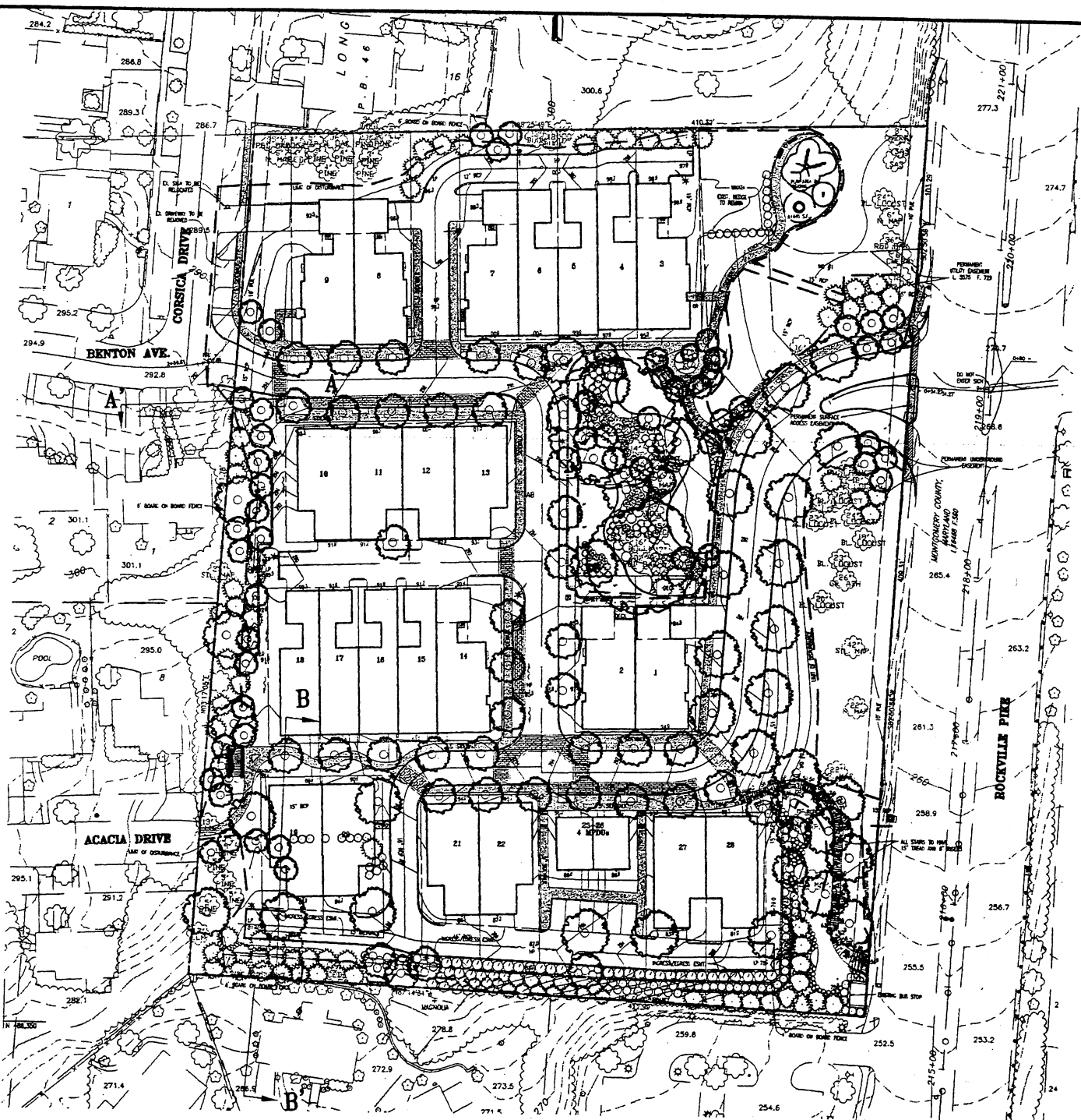
PLAN VIEW (R-60 MPDU)
