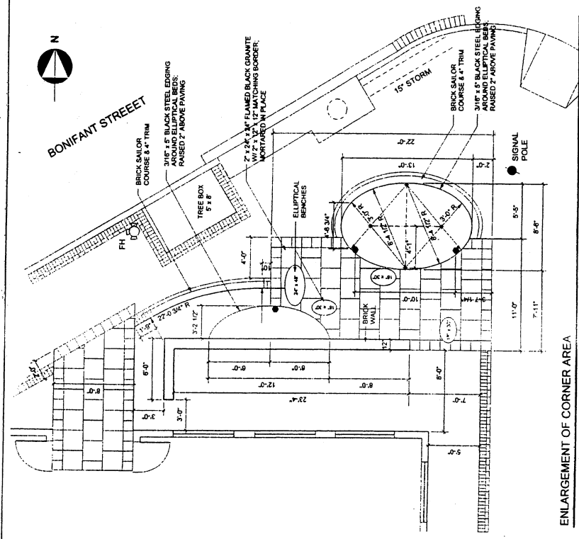
PAVING & TREE BOX ALONG BONIFANT STREET SCALE: 1/2" = 1'-0"
