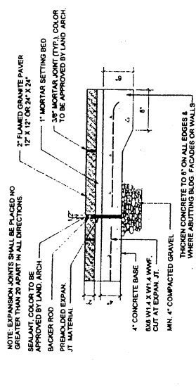
TYPICAL SECTION - GRANITE PAVING MORTARED-IN-PLACE SCALE: 1/2" = 1'-0"
