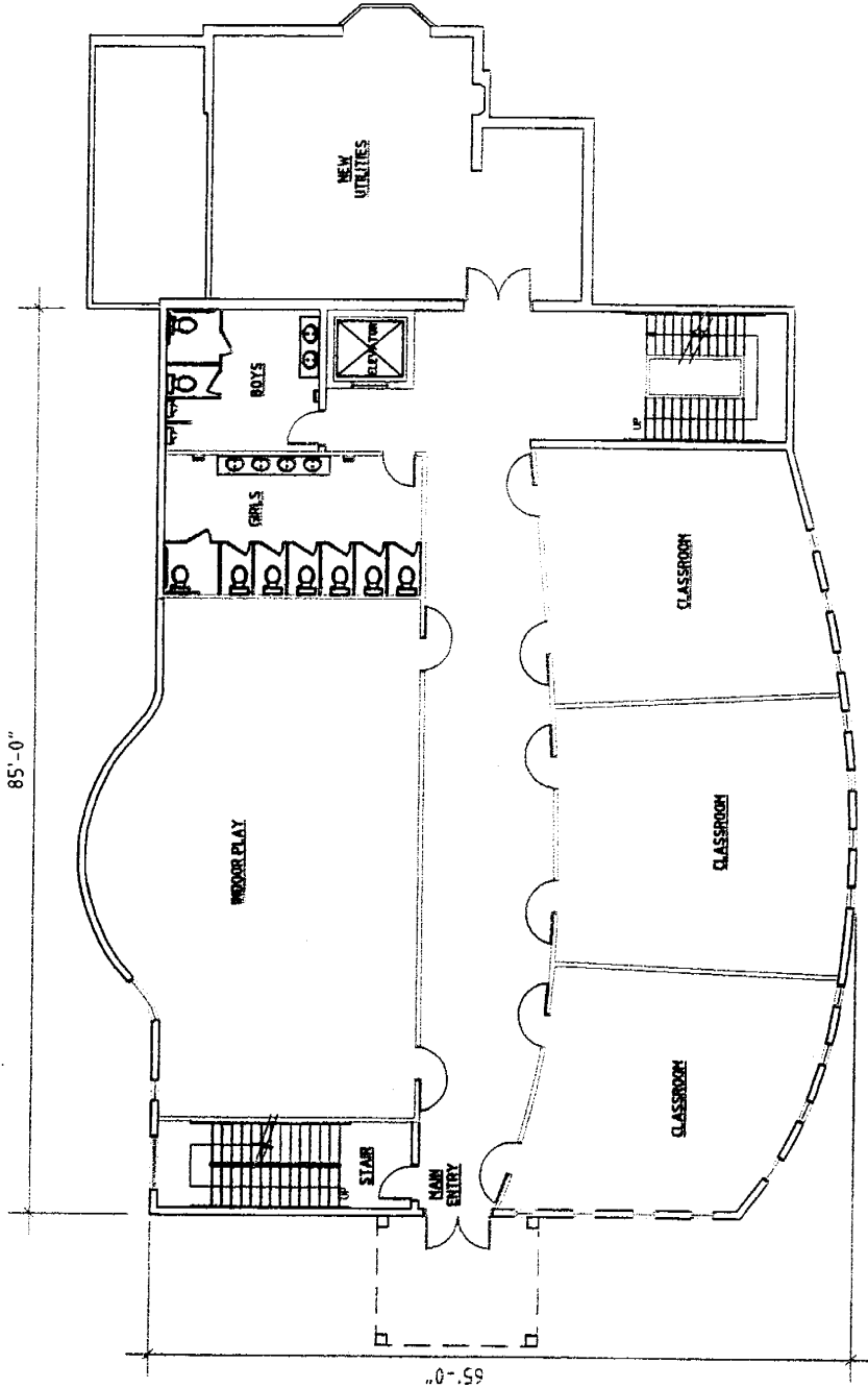
LOWER LEVEL PLAN (5,525 SF)
